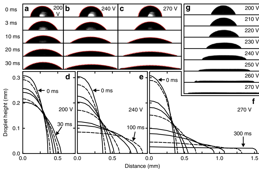
Figure 2 | Dynamic drop shape profiles at different spreading voltages. (a-c) show actual drop shape profiles viewed from the y-direction and (d-f) show digitized drop shape profiles. The profiles are shown as a function of time after a constant amplitude sine wave voltage (10 kHz) is applied to the electrodes: a and d just below the threshold voltage (200 V, V/V_{Th} = 0.87 ); b and e just above the threshold voltage (240 V, V/V_{Th} = 1.04 ); and c and f further above the threshold voltage (270 V, V/V_{Th} = 1.17 ). In panels d-f digitized profiles are shown at times 0, 1 ms (dashed), 3 ms, 5 ms, 10 ms (dashed), 30 ms, 50 ms, 100 ms (dashed) and 300 ms. The red dashed lines shown in a-c are fits to circular arcs. ( g ) Shows equilibrium (long time limit) droplet shapes viewed from the y-direction for a range of different spreading voltages from 200 to 270 V. The vertical scale in g is expanded by a factor of 2 compared with the horizontal scale so that the spread film at 270 V can be clearly seen.
