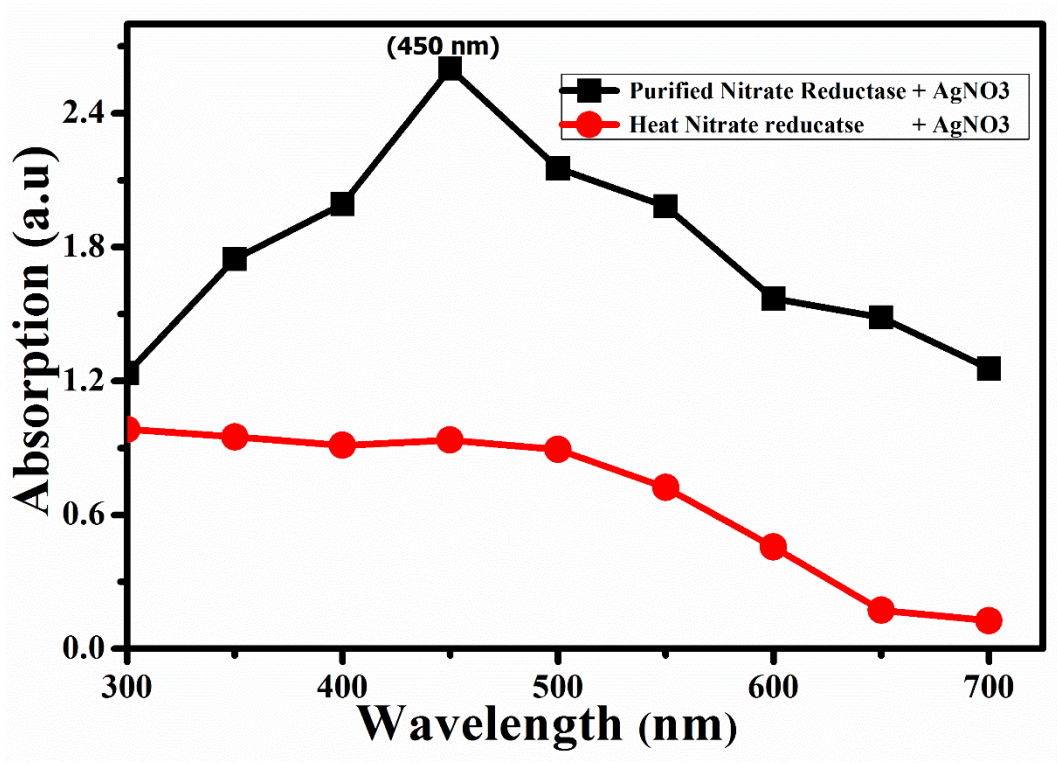
Figure.7 .UV-Visible spectrum of reaction mixtures containing the purified enzyme and AgNO3 solution.
