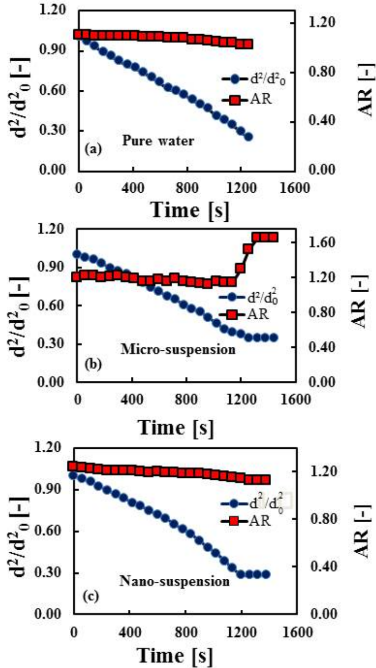
Figure 5. The measured equivalent diameter, d , and aspect ratio ( AR ) of a) pure water b) 1% micro-suspension (radius of 2.5 \mu\text{m} ) and c) 1% nano-suspension (radius of 8 \text{ nm} ) droplets with an initial droplet volume of 2.3 \mu\text{l} . d_0 corresponds to the initial droplet diameter.
