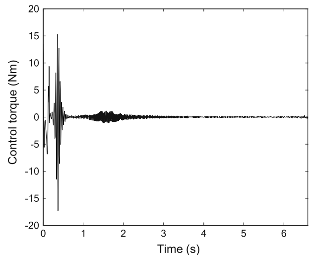
Fig. 12 Control torque
