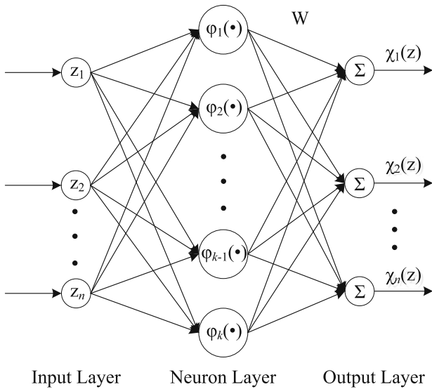
Fig. 1 Structure of the RBFNN
