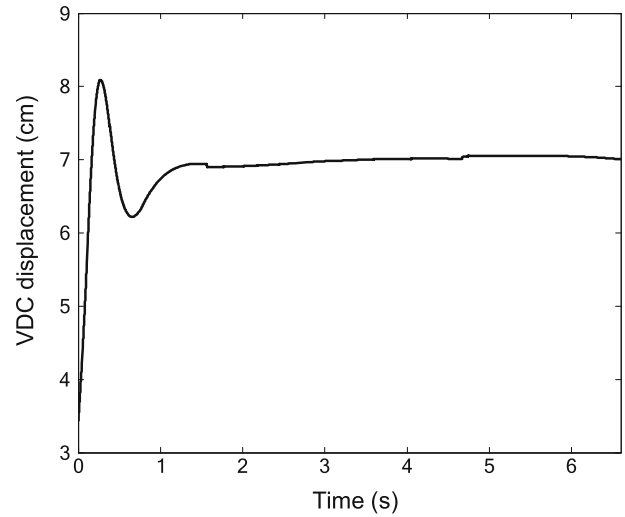
Fig. 11 Performance of the vibro-driven system
