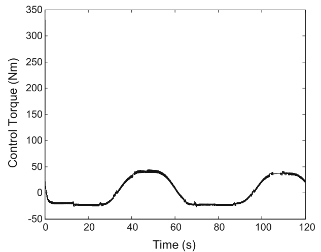
Fig. 5 Control input torque
