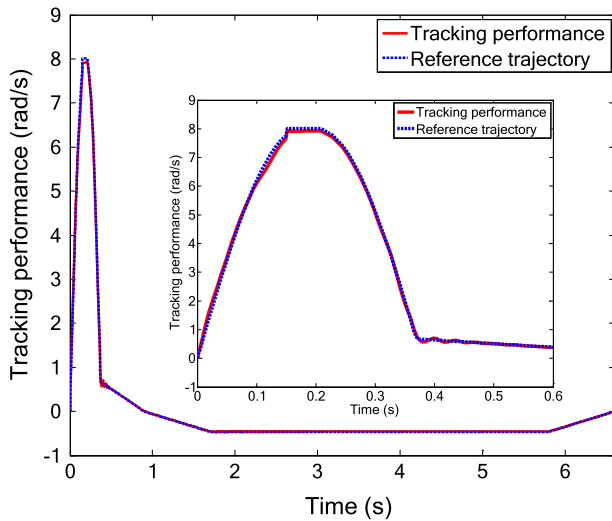
Fig. 9 Trajectory tracking performance
