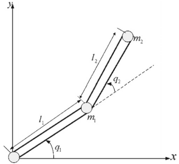
Fig. 2 The 2-DOF underactuated manipulator
