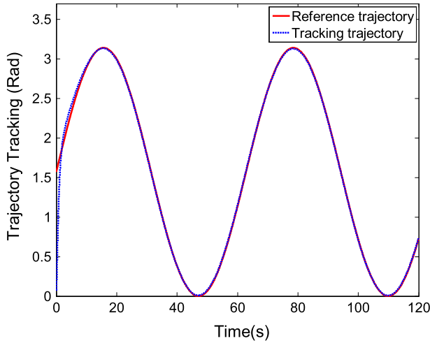
Fig. 3 Trajectory tracking performance
