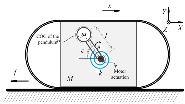
Fig. 8 Schematic of the underactuated vibro-driven system
