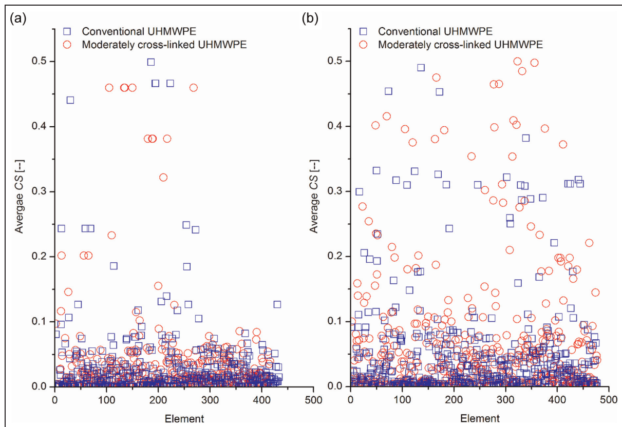
Figure 6. Effect of insert bearing material on the predicted average elemental CS for the Sigma curved insert under (a) intermediate and (b) high kinematic inputs.
