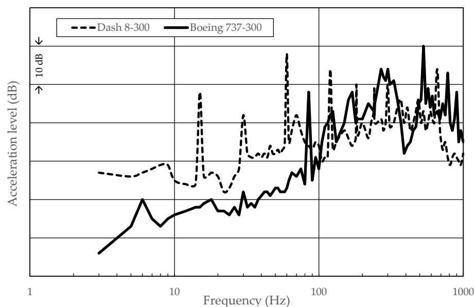
Figure 1. Typical vibration measured at the seat rail in the vertical direction for a turboprop (Dash 8) and jet aircraft (737) during the cruise phase (adapted from [25]). NB absolute values are not reported in the source.
