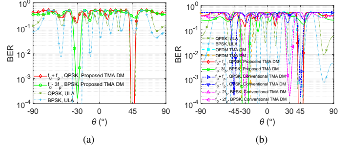
Fig. 4. The BERs of various DM schemes. (a) SNR=10dB. (b) SNR=15dB.
