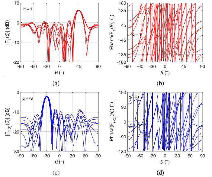
Fig. 2. Far-field radiation patterns. (a), (c) magnitudes in dB; (b), (d) phases in degrees; at frequencies of f_0 + f_p , f_0 - 3f_p , respectively.
