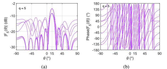
Fig. 3. Far-field radiation patterns. (a) magnitudes in dB; (b) phases in degrees; at frequency of f_0 + 5f_p .
