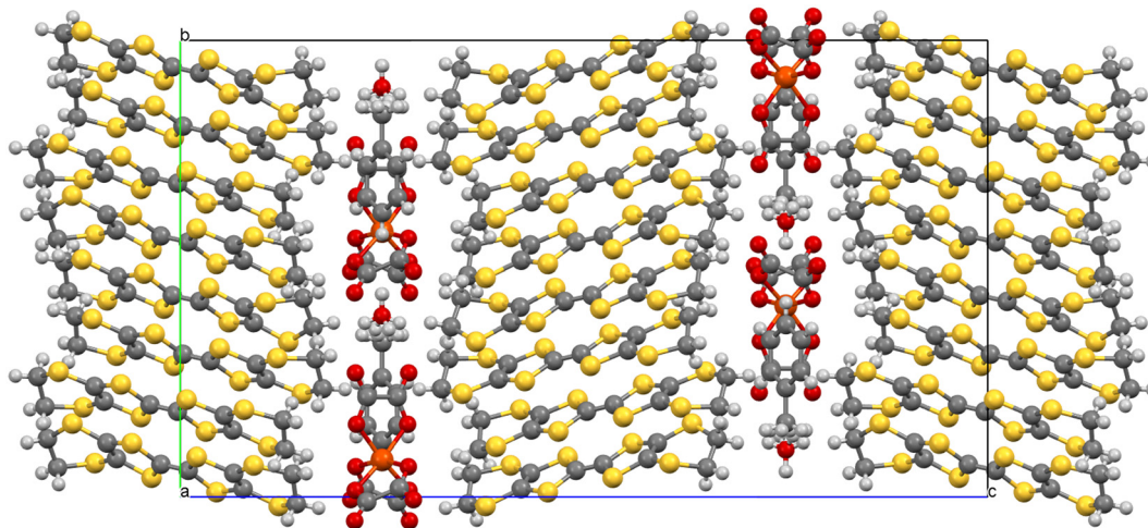
Fig. 1 \beta'' -(BEDT-TTF) _4 [(H _3 O)Fe(C _2 O _4 ) _3 ]·toluene (I) viewed down the a axis.
