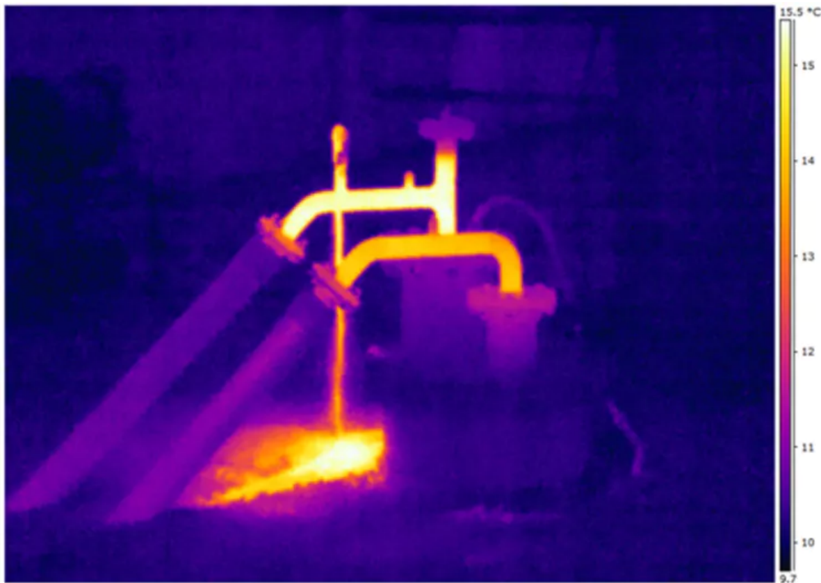
Infrared image showing the warm water pumped from flooded coalmine. Author provided (No reuse)
