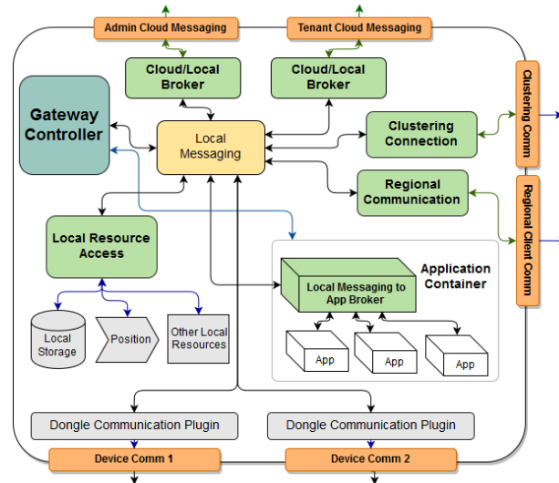
Fig. 1. Architecture of the Gateway
