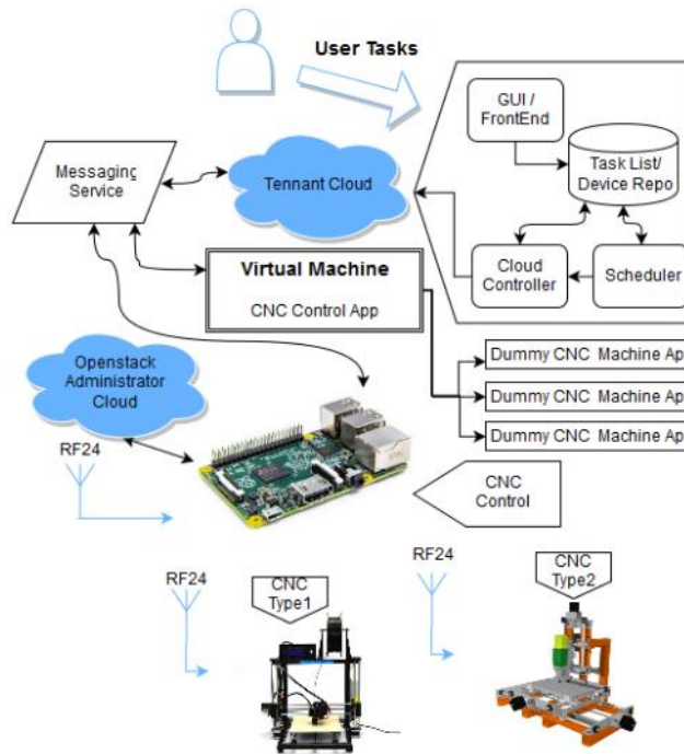
Fig. 5. Overview of Orchestration system
