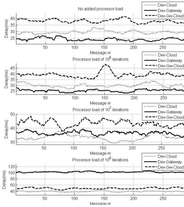
Fig. 8. Processor Load based Response Time
