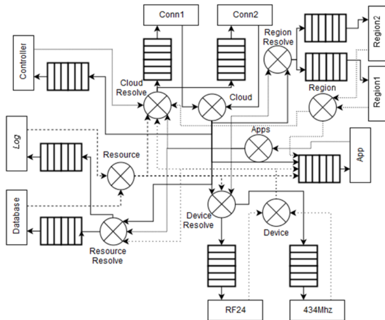
Fig. 2. Messaging Exchanges and routing
