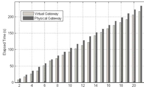
Fig. 7. Virtual and Physical task processing
