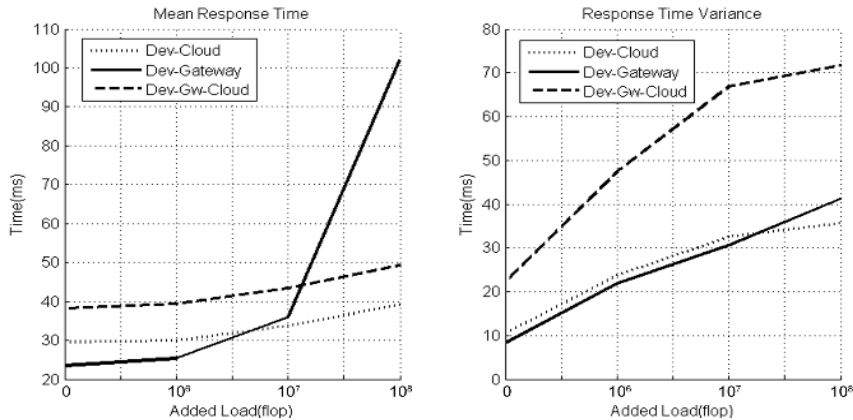
Fig. 9. Response times and variance
