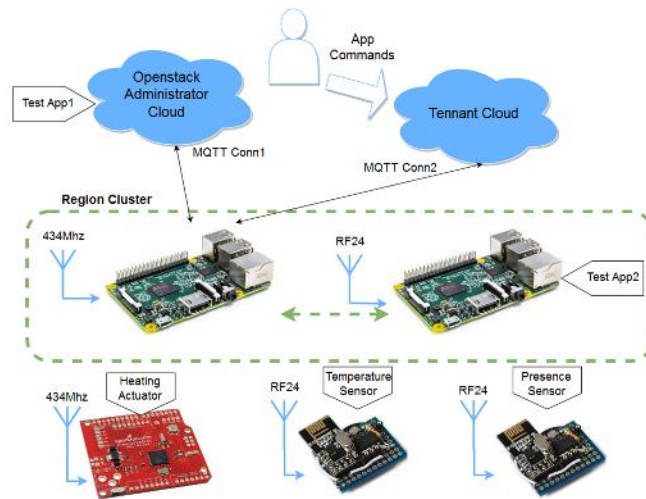
Fig. 4. Control and Metering Application
