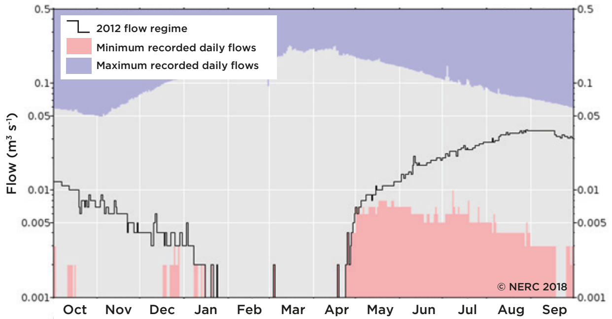
Figure 3: Daily flow on Ewelme Brook, a chalk river in south England
