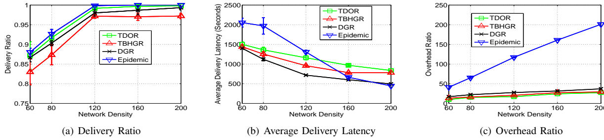
Fig. 7. Influence of Network Density
