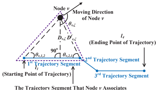
Fig. 3. An Example of Trajectory Association
