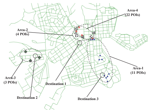
Fig. 5. Evaluation Scenario
