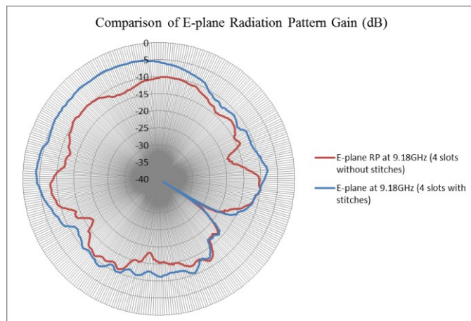
Fig.4.(a) Comparison of E-plane radiation pattern
