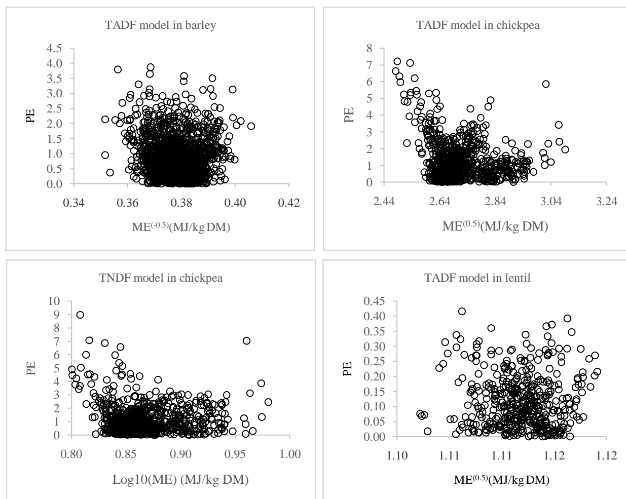
Figure 3 Relationship between the dependent variable and prediction error of constructed models of barley, chickpea and lentil training straw samples.
