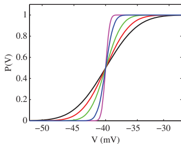
Figure 1. The probability of firing in a model with Gaussian threshold noise. Here V_{th} = -40 mV and \sigma = 4 mV -1 (black), \sigma = 3 mV -1 (red), \sigma = 2 mV -1 (green), \sigma = 1 mV -1 (blue) and \sigma = 0.5 mV -1 (magenta).
