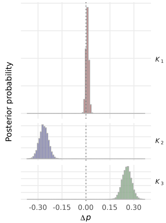
Fig. 2: Posterior probability of NP type difference of mixing proportions \Delta \rho = conjoined NP - simple NP by K .
