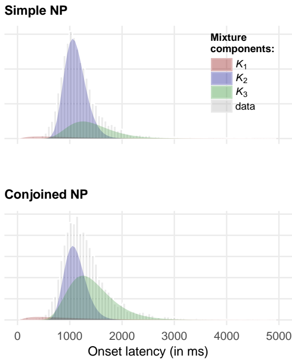
Fig. 1: Posterior distributions of mixture components inferred from M2.
