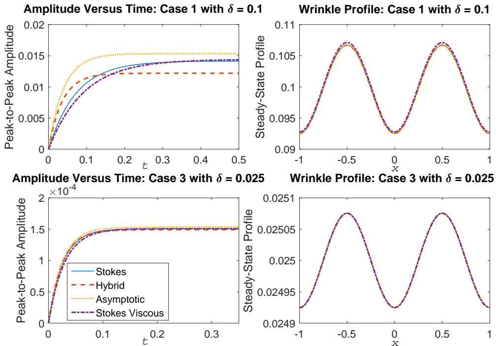
FIGURE 3. The time evolution of the wrinkle amplitude from flat to steady-state (left column) and the final steady-state wrinkle profile (right column). The rows represent the thinnest film experiment shown in Figure 2 for two of the three forcing cases: Case 1 with \gamma = \epsilon_0/50 and case 3 with \gamma = \epsilon_0/5000 . The dash-dot curve (Stokes Viscous) shows the effect of reducing the viscosity ratio between \Omega_1 and \Omega_2 in the Stokes flow boundary integral model from 10^4 to 2.
