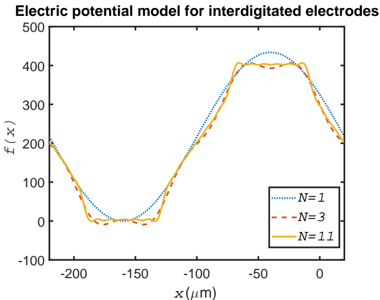
FIGURE 5. Modelling the electric potential from an array of interdigitated electrodes using equation (6.3) with parameters \Phi = 400V , L = 240\mu\text{m} and truncating the sum after N terms as specified in the legend.
