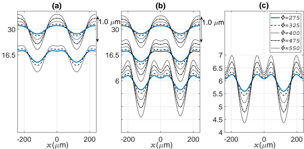
FIGURE 6. The steady-state wrinkle profile of a hexadecane oil-air interface predicted by (a) the Stokes flow numerical model, (b) the hybrid numerical asymptotic model and (c) the fully asymptotic model. The mean film height h_0 is chosen as h_0 = 6\mu\text{m} , 16.5\mu\text{m} , 30\mu\text{m} , corresponding to a small parameter \delta ranging from 0.025 to 0.125, and results for each model are presented in appropriate regimes (see text). A simulated array of interdigitated electrodes is applied to excite the system via equation (6.3) and truncating the sum after three terms. The applied potential is indicated in the legend of the right sub-plot, and is consistent throughout all subplots. The plots are all scaled consistently, but their position on the vertical axis has been shifted for ease of comparison between different values of h_0 .
