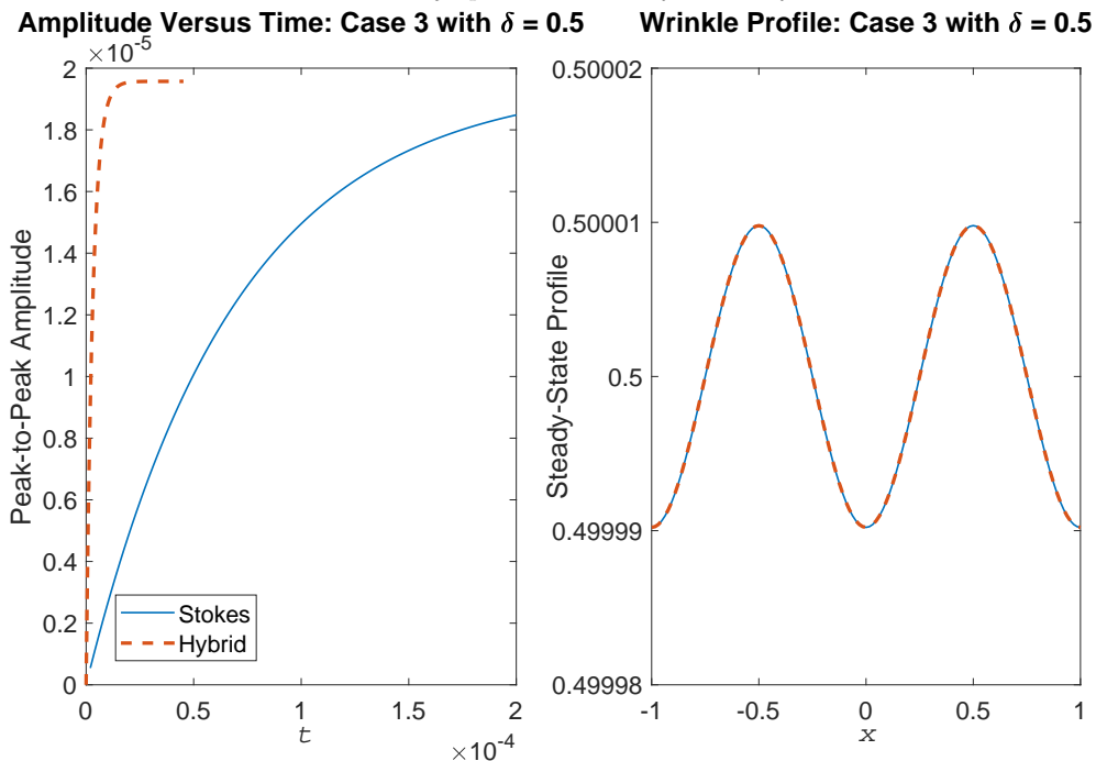
FIGURE 4. The time evolution of the wrinkle amplitude from flat to steady-state (left column) and the final steady-state wrinkle profile (right column) for a thick film with \delta = 0.5 and \gamma = \epsilon_0/5000 .
