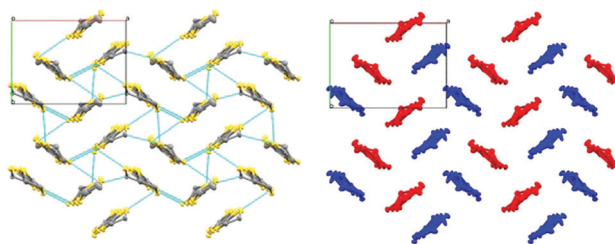
Fig. 5 \kappa -Type packing, with short contacts shown as blue dashed lines (left) and the crystallographically independent donors shown in red and blue (right). Thermal ellipsoids set at 50% probability, hydrogen atoms and minor disordered components omitted for clarity.
