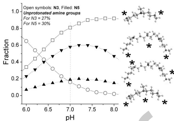
Fig. 4 Estimated speciation of N3 and N5 (only species present at significant fractions are shown). Models of propylamines are shown on the right of each curve. Nitrogen atoms in red are charged.
