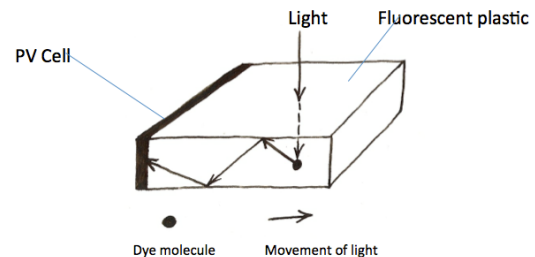
Figure 1: The principle of light collection via an LSC.
