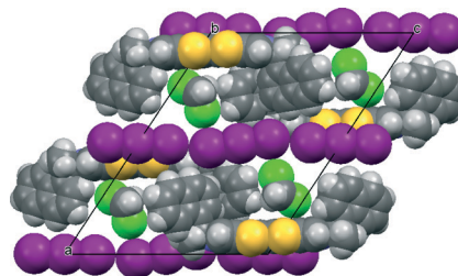
Fig. 8 Crystal packing of 12 \cdot I_3 \cdot CH_2Cl_2 viewed down the b axis with one orientation for the triiodide and associated dichloromethane molecule.
