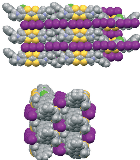
Fig. 7 Crystal packing in 12 \cdot I_3 \cdot chlorobenzene viewed on the bc plane (above) and viewed along the c axis (below).
