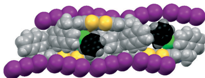
Fig. 6 View of the structure of 12 \cdot I_3 \cdot chlorobenzene, showing how the solvent molecules lie close to the interface between triiodide ions.
