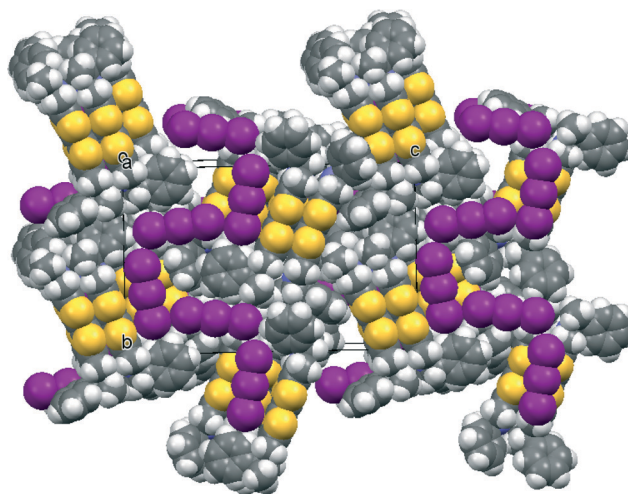
Fig. 9 Packing arrangement of 13 \cdot I_3 viewed in the bc plane showing the castellated arrangement of triiodide ions. Note that the apparent space between the castellated triiodides and phenyl groups is filled by phenyl rings from the next layer above.
