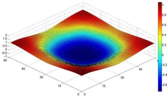
Mode Shape 2
