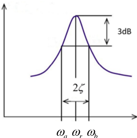
Fig. 4 FRF plot for extracting damping ratio
