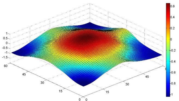
Mode Shape 3
