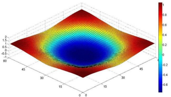
Mode Shape 2
