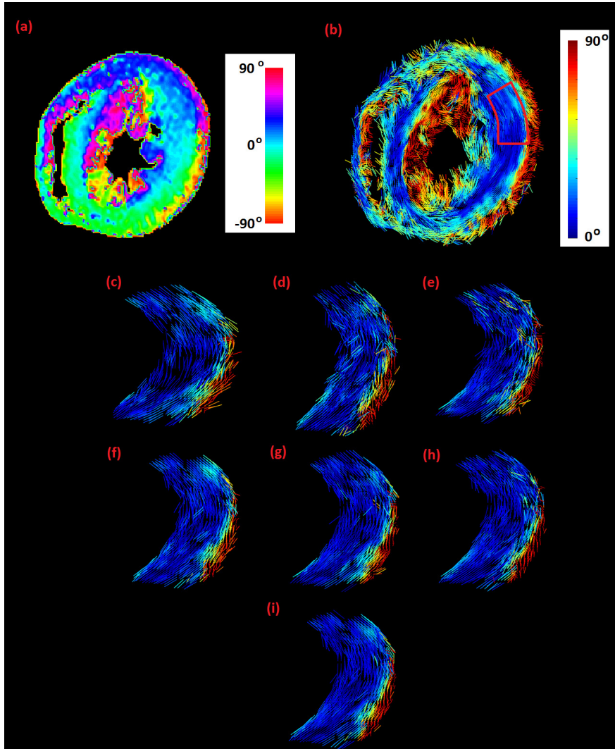
Figure 6: (a) Helix angle map, where helix angle is defined (Streeter et al., 1969) as the angle between the cardiac short-axis plane and the projection of the primary eigenvector onto the epicardial tangent plane. (b)-(i) Images of the primary eigenvector field, color encoded to the absolute local helix angle. (b) The whole equatorial short-axis slice. The red sector indicates the zoom-in area (lateral wall). Remaining images are close-ups that refer to the 1st acquisition (c), 2nd acquisition (d), 3rd acquisition (e), mean of the 1st and 2nd acquisitions (f), mean of the 1st and 3rd acquisitions (g), mean of the 2nd and 3rd acquisitions (h), mean of all three acquisitions (i). The tensor averaging impact is the realignment of some primary eigenvectors that had atypical directions due to noise. Results are shown when the Log-Euclidean distance function was used for tensor averaging. Similar results were obtained for the other two studied distance functions.
