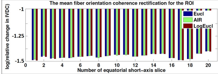
Figure 3: The directional regularity restoration performance of the Euclidean (Eucl), log-Euclidean (logEucl) and affine-invariant Riemannian (AIR) distance functions as assessed by the logarithmic relative change in the IVDC index before and after averaging for the five hearts. Results are presented over 20 short-axis slices of one rat heart of this study. The 20 slices spanned the whole 3D acquisition volume.
