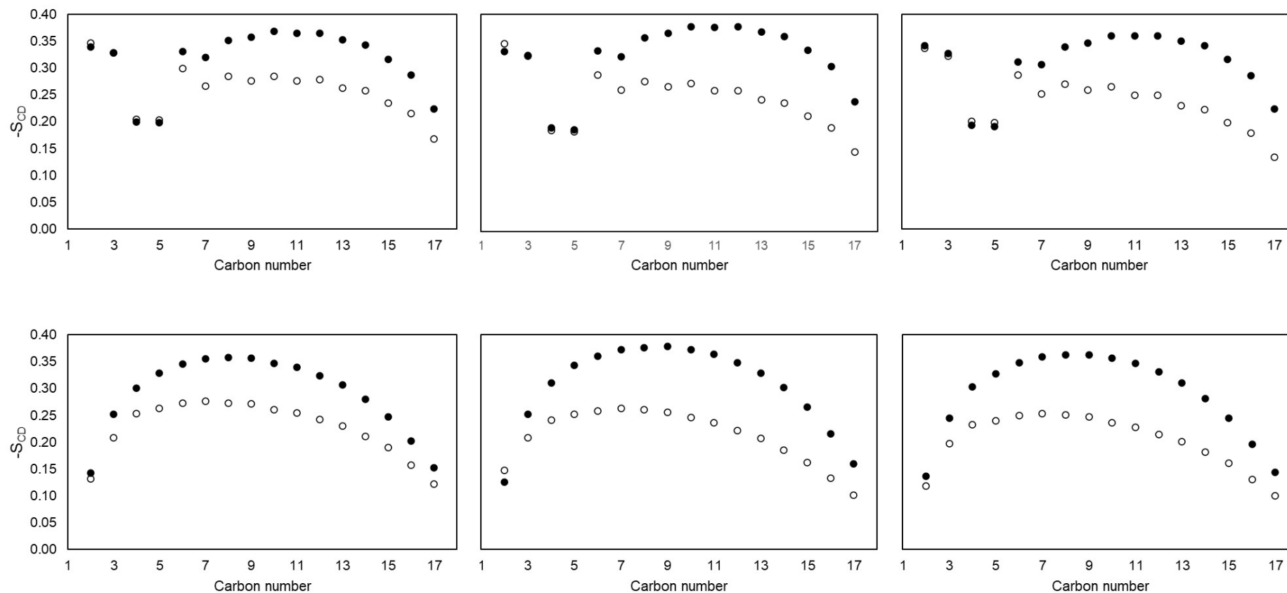
Figure 4. Calculated deuterium order parameters for SSM for the sphingosine chain (top) and stearyl chain (bottom) at 310 K (left), 320 K (middle) and 330 K (right). Filled circles are from the SSM/cholesterol simulation; open circles taken from the SSM-only simulation.
