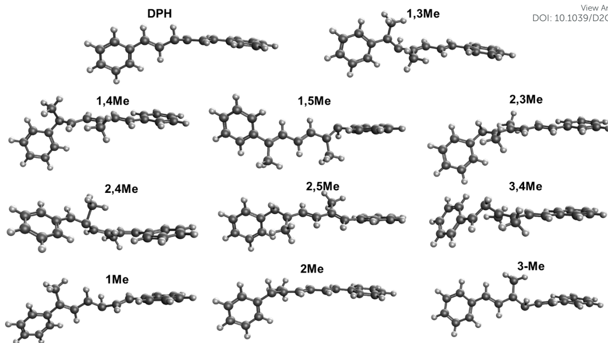
Figure 2. MECl geometries calculated using SF-TDDFT and full analytical non-adiabatic couplings using the BHHLYP functional and 6-31G(d,p) basis set.
