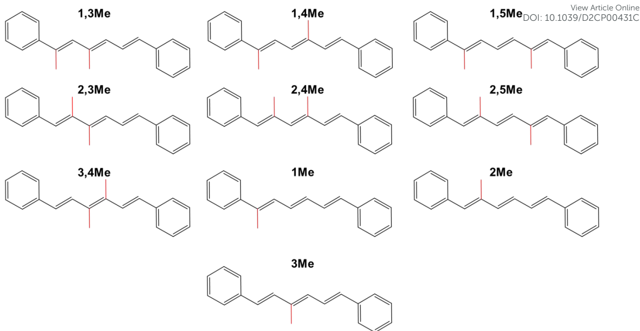
Figure 1. Molecular structures of the 1,6-diphenyl-1,3,5-hexatriene derivatives considered in this work, along with the abbreviated names used throughout this study.
