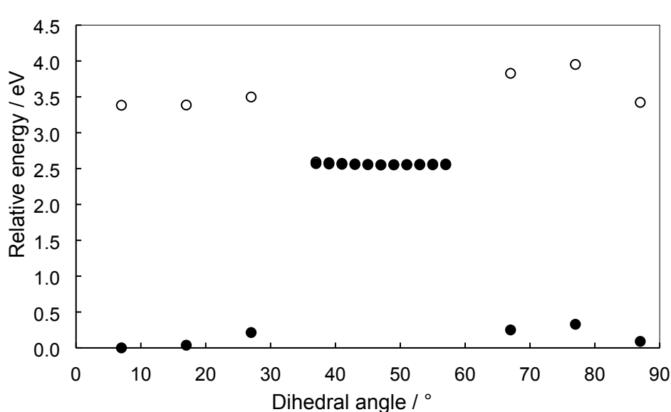
Figure 3. Scan of the S_0 (filled circles) and S_1 (open circles) reaction coordinate of the S_1 electronic state through the MECI of 2Me using values of the C1-C6-C7-C8 dihedral angle, using BHHLYP/6-31G(d,p). S_1 energies were calculated within the SF-TDDFT formalism. Geometries for each point were taken from a reaction pathway calculation calculated along the S_1 potential energy surface.
