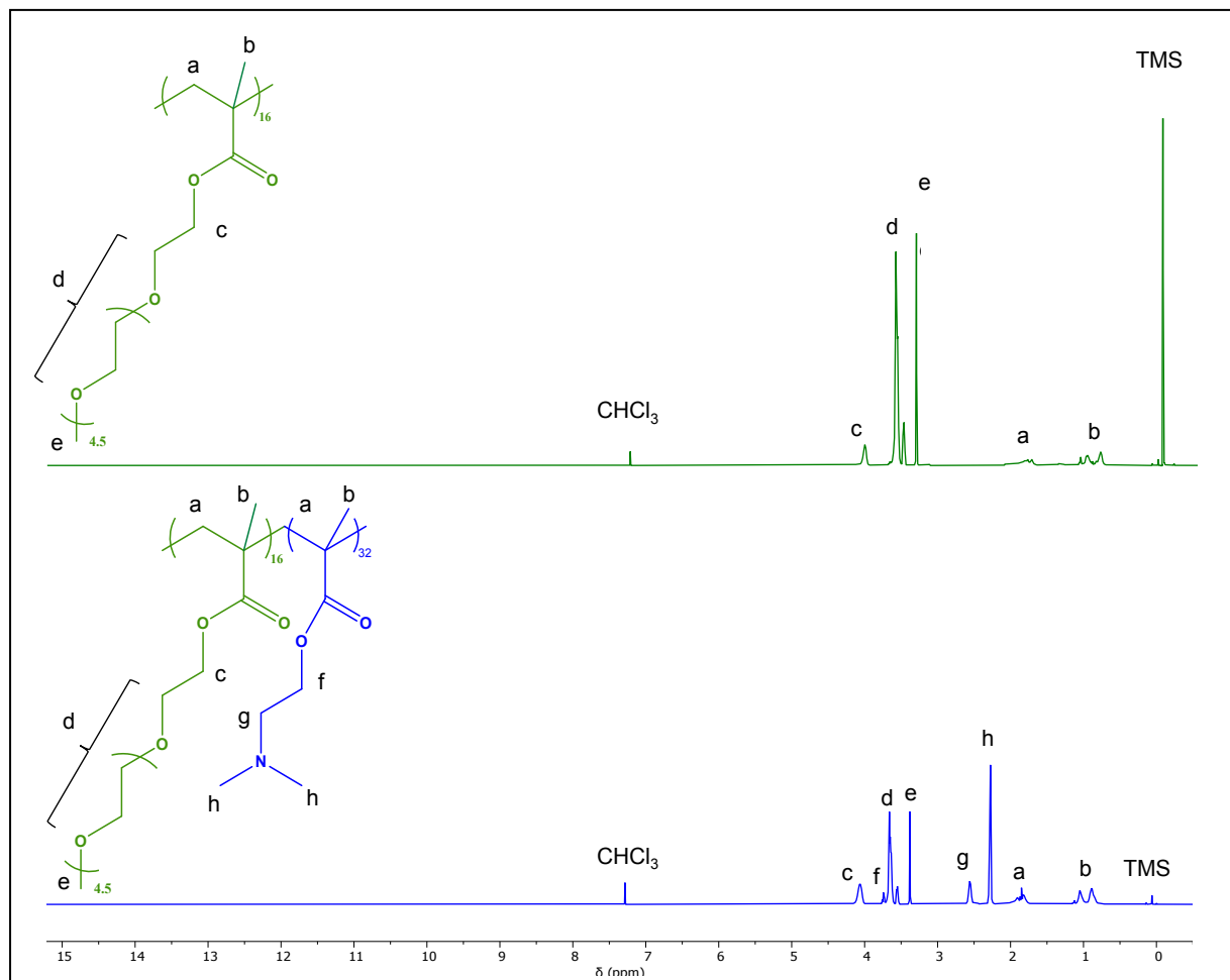
Figure 3. ^1\text{H} NMR spectra of the AB diblock copolymer, OEGMA300 16 - b -DMAEMA 32 (P1), and its precursor. The first block of the copolymer, OEGMA300, is represented in green (chemical structure and spectra), the second block, DMAEMA, is represented in bright blue (chemical structure), and the final spectra in bright blue.
