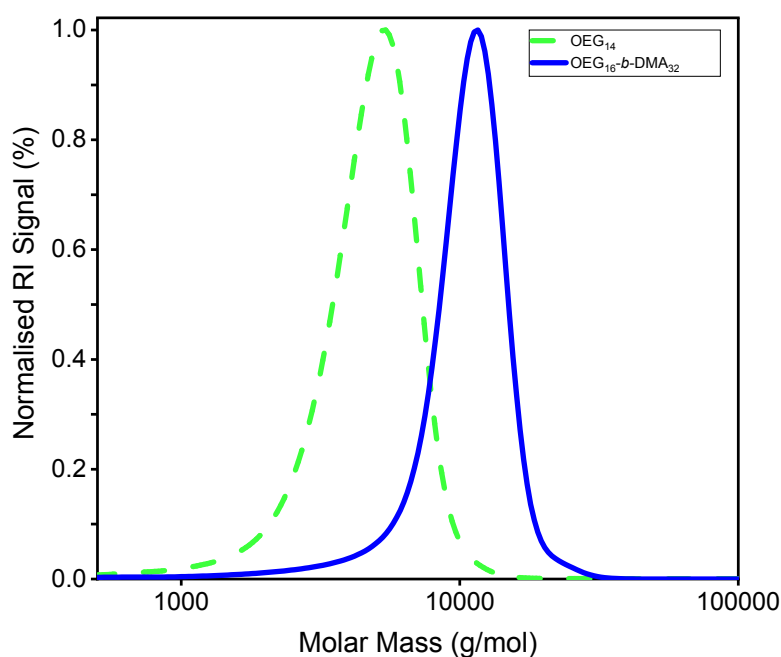
Figure 2. GPC chromatogram of the AB diblock copolymer, OEGMA300 16 - b -DMAEMA 32 (P1), and its precursor, OEGMA300 14 (abbreviated OEG 14 on inset legend) and the final polymer (abbreviated OEG 16 - b -DMA 32 on inset legend) are represented by the green dashed line and blue solid line, respectively.
