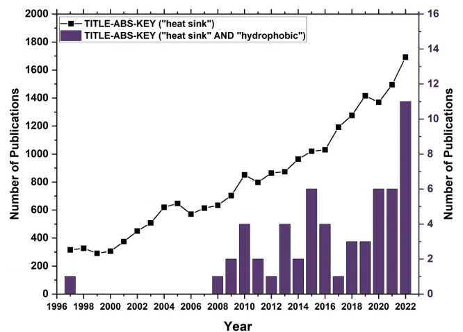
Fig. 1. Comparative Analysis of Research Publications on Heat Sinks over the past 25 years (Scopus database).
