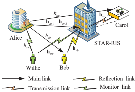
Fig. 1. System model of STAR-RIS NOMA network.
