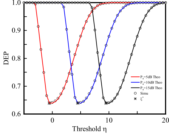
Fig. 2. DEP versus \eta for the comparison of different P_a .
