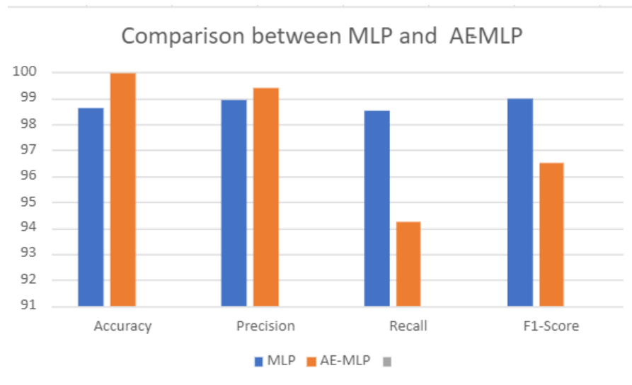
Figure 10. Hybrid Autoencoder–Multi-Layer Perceptron (AE–MLP) model comparison with Multi-Layer Perceptron (MLP).
