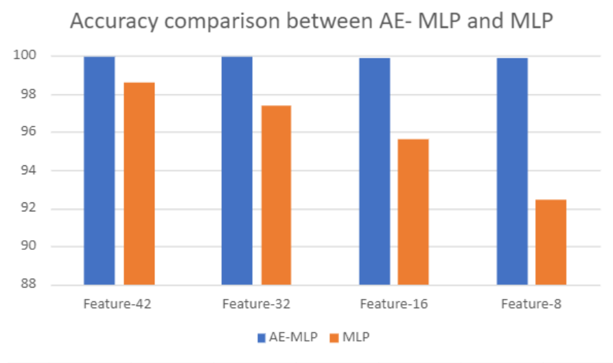
Figure 11. Feature hybrid Autoencoder–Multi-Layer Perceptron (AE–MLP) model comparison with Multi-Layer Perceptron (MLP).
