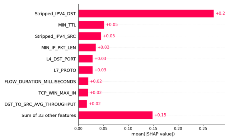
Figure 4. Mean absolute value to determine feature importance.
