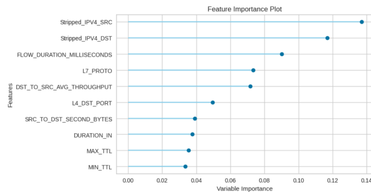
Figure 2. Feature importance result.
