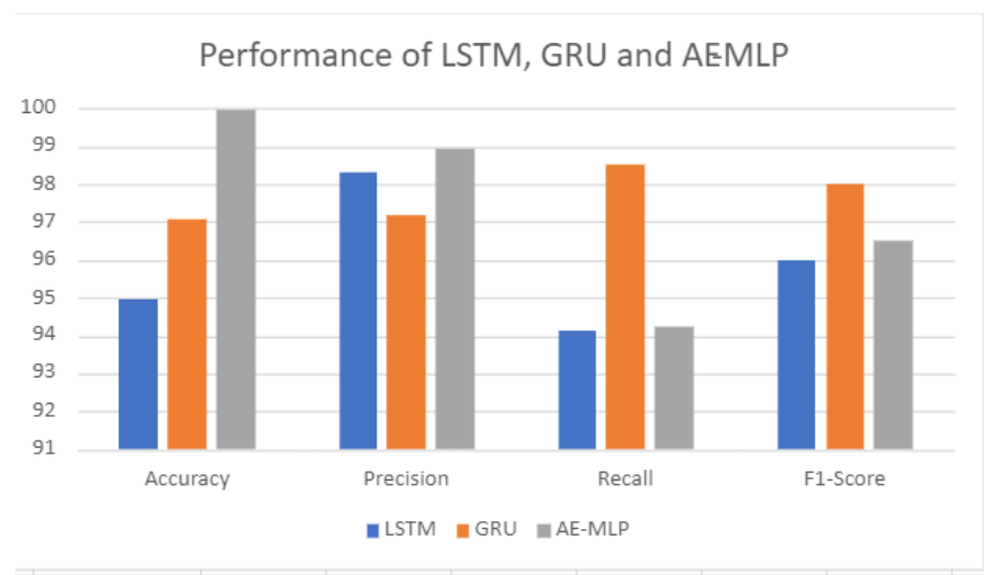
Figure 9. Comparison between Long Short-Term Memory (LSTM), Gated Recurrent Units (GRU), and the hybrid Autoencoder–Multi-Layer Perceptron (AE–MLP) model.
