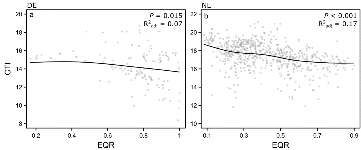
Supplementary Fig. 6: Relationship between the Ecological Quality Ratios (EQRs) and the Community Temperature Index (CTI) in (a) Germany (DE) and (b) the Netherlands (NL).
