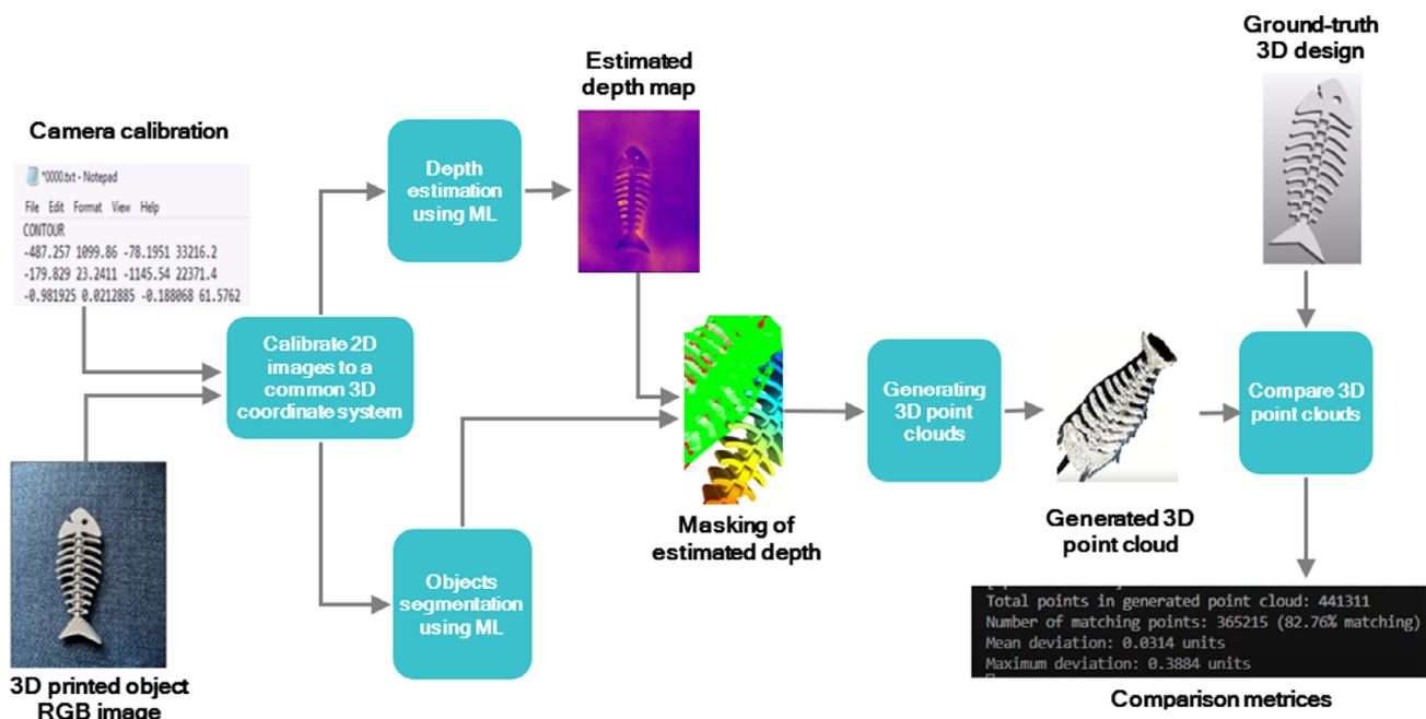
Figure 16. A case study of a ML pipeline for assessing the geometric accuracy of a 3D-printed object via RGB image-based reconstruction and point cloud comparison to the CAD model.
